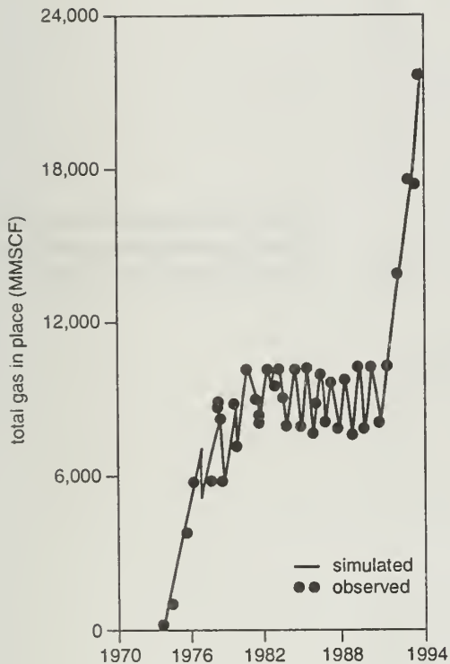
Figure 10 History match of the total Hillsboro Field gas-in-place inventory.
